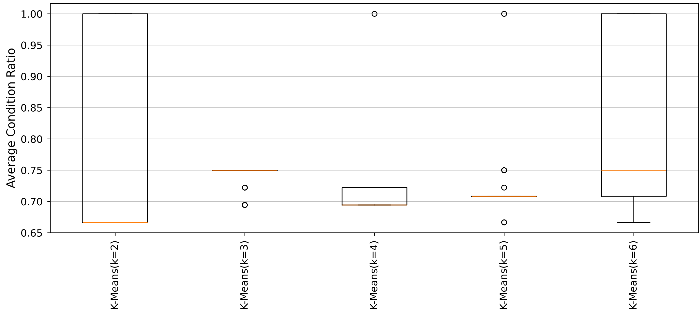
YARA Rules Average Condition Ratio Distribution (Cluster33_Size6 dataset)
